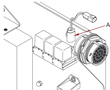
Series MO
